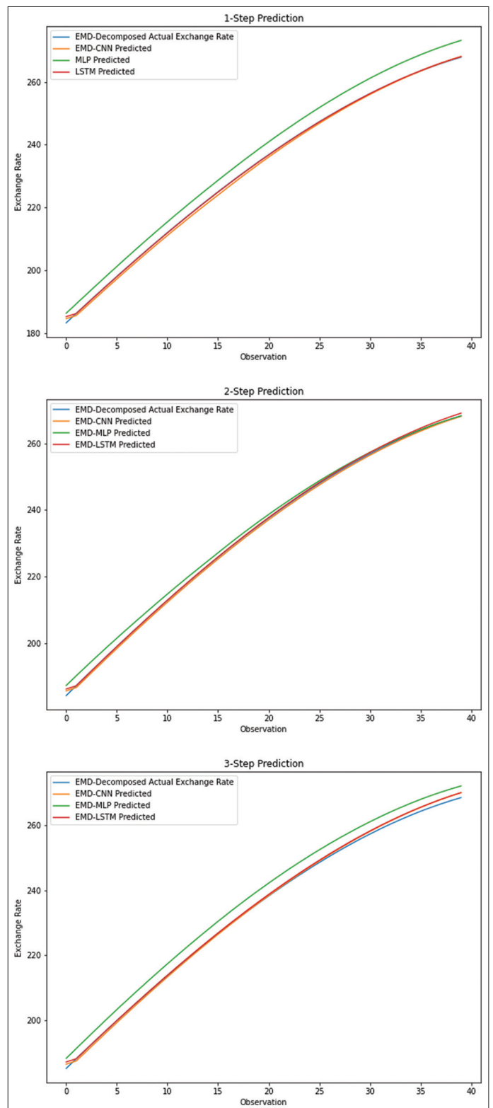
Figure 7: Comparison of Multivariate (Decomposed) deep models
